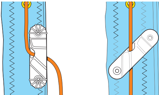
B301 alternative position. Typical mainsail reef application
