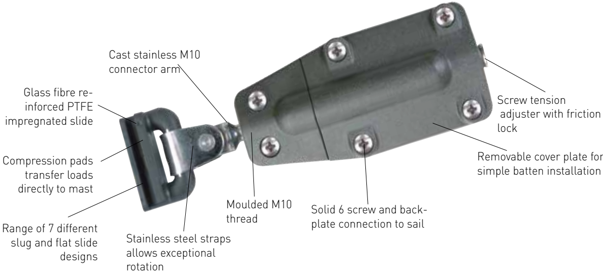
Series 25 (U01540) Luff Box Shown
